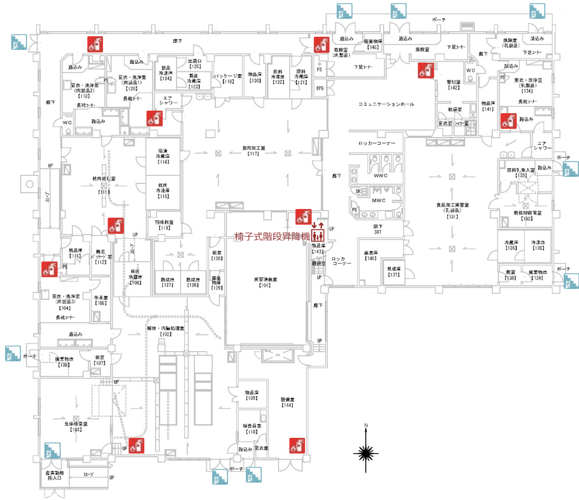
Food Processing Practice Facility 1st Floor
