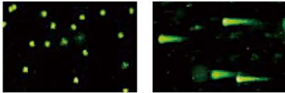
The nuclei of malarial protozoa infecting the red blood cells of a wild-type mouse (A). Disturbances in the DNA of protozoa infecting the red blood cells of an \alpha -TTP deficient mouse (B).
