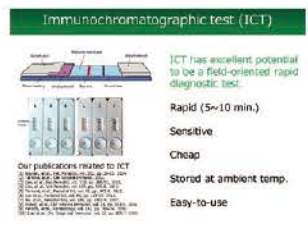
Immunochromatography for the diagnosis of protozoan diseases
