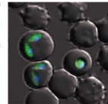
Genome editing by CRISPR/Cas9 system
